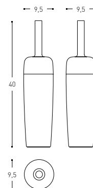
● ▲ 258 AA 00 ESCOBILLERO TOILET BRUSH PORTE-BALAYETTE PORTASCPINO PORTA-PIACABA TOILETTENBÜRSTENHALTER WC-BORSTELHOUDER
